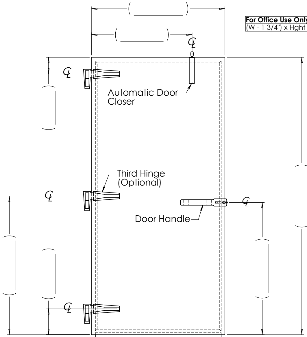
EXTERIOR VIEW (View Shown As Hinged Left)
